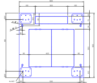
Drawing of the roof of a 600 mm wide RMA cabinet.
